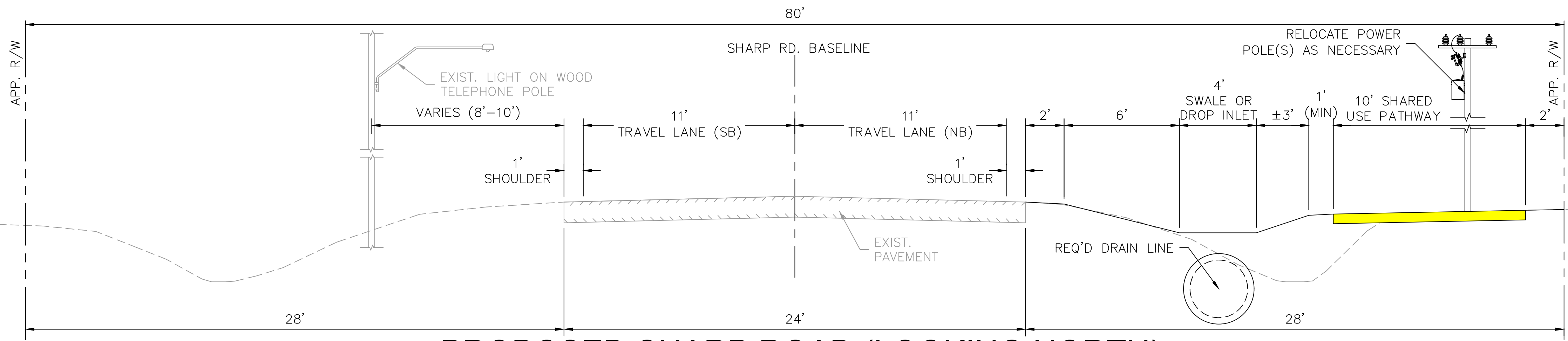
PROPOSED SHARP ROAD (LOOKING NORTH) CLASSIQUE DR. TO MOLLYLEA DR.
