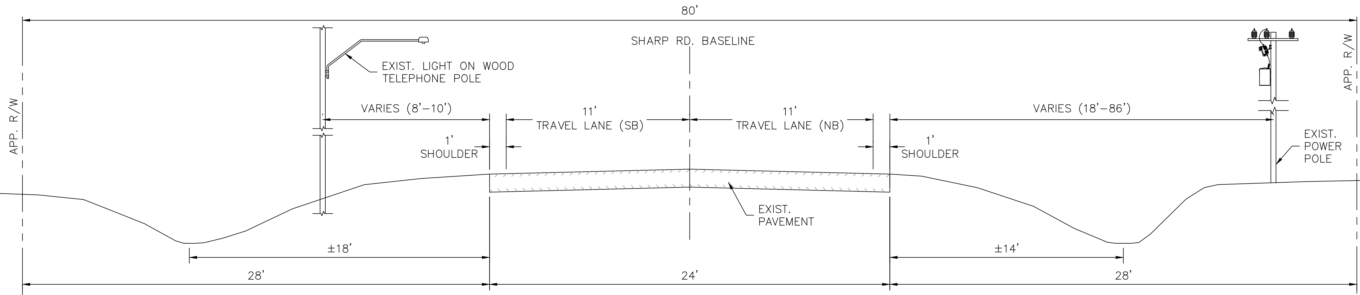
EXISTING SHARP ROAD (LOOKING NORTH)
