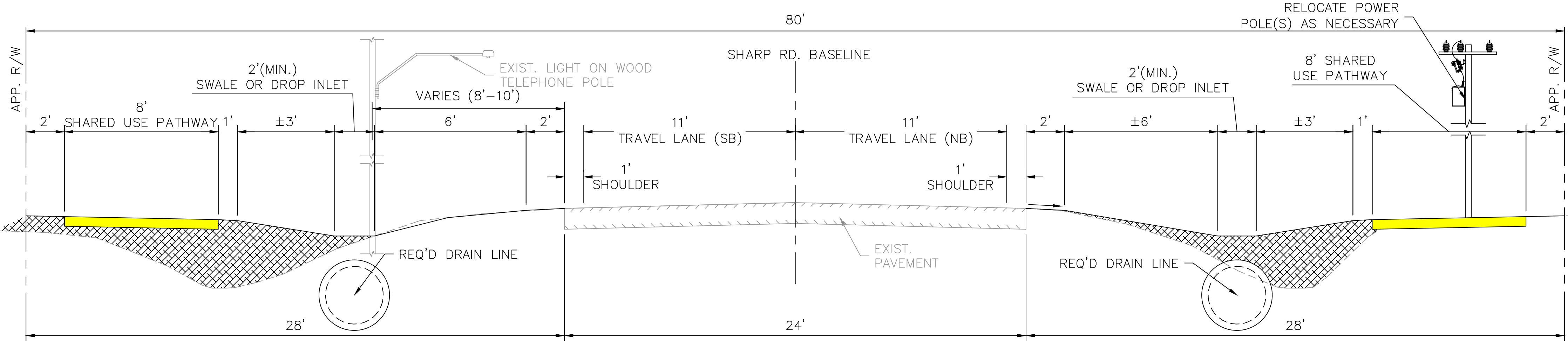
PROPOSED SHARP ROAD (LOOKING NORTH) MOLLYLEA DR. TO FLORIDA BLVD.
