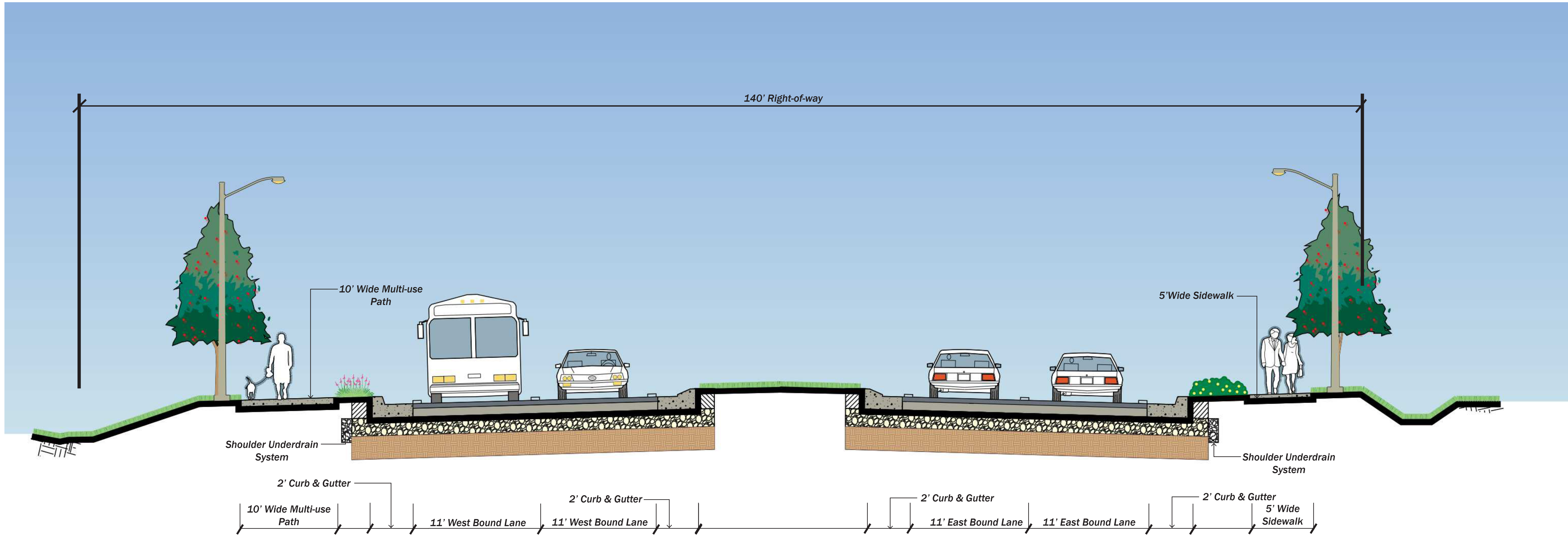
Typical Section - Proposed Improvements
