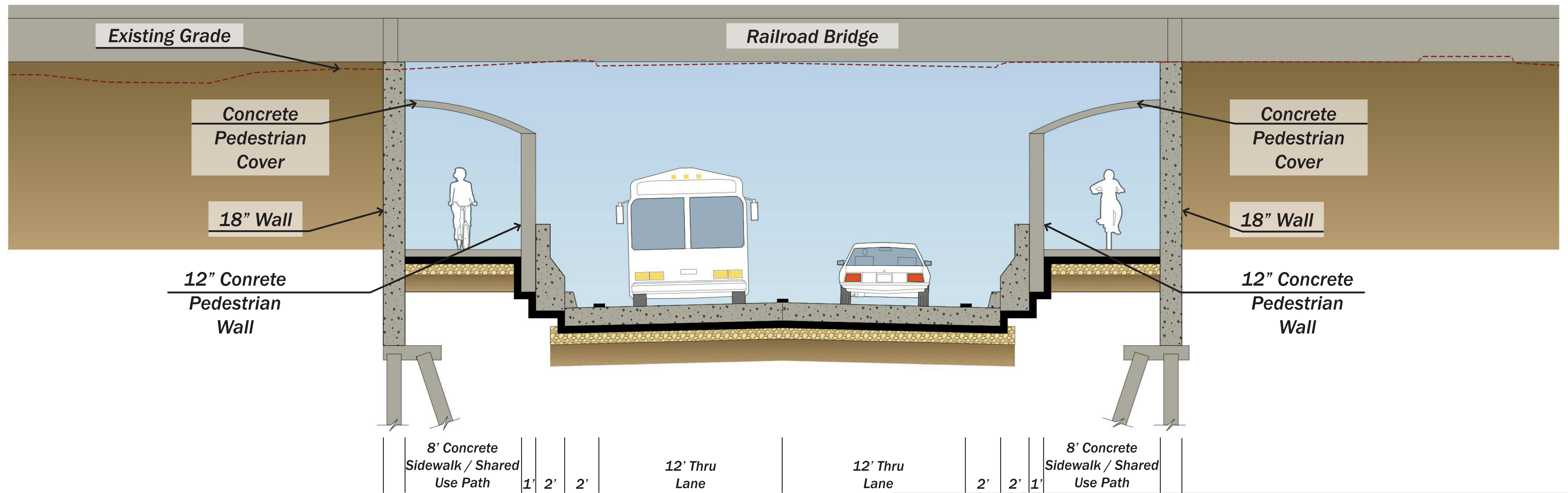
Elevation B-B - Not to Scale, for Illustration Purposes Only
