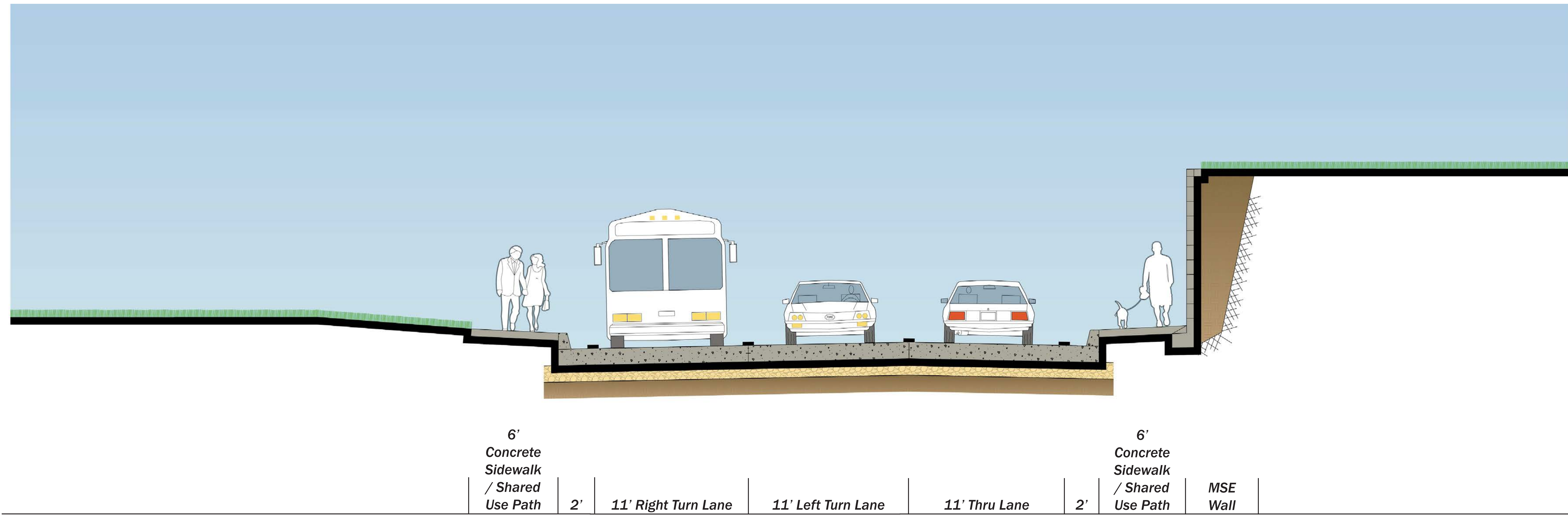
Elevation E-E - Not to Scale, for Illustration Purposes Only
