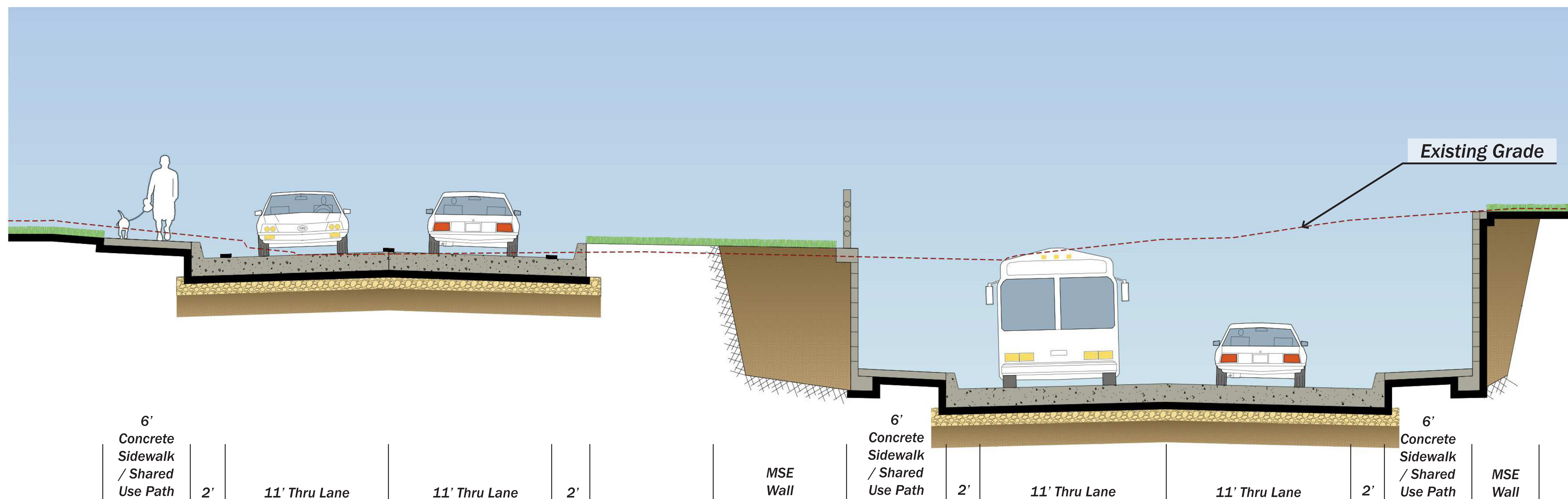
Elevation D-D - Not to Scale, for Illustration Purposes Only
