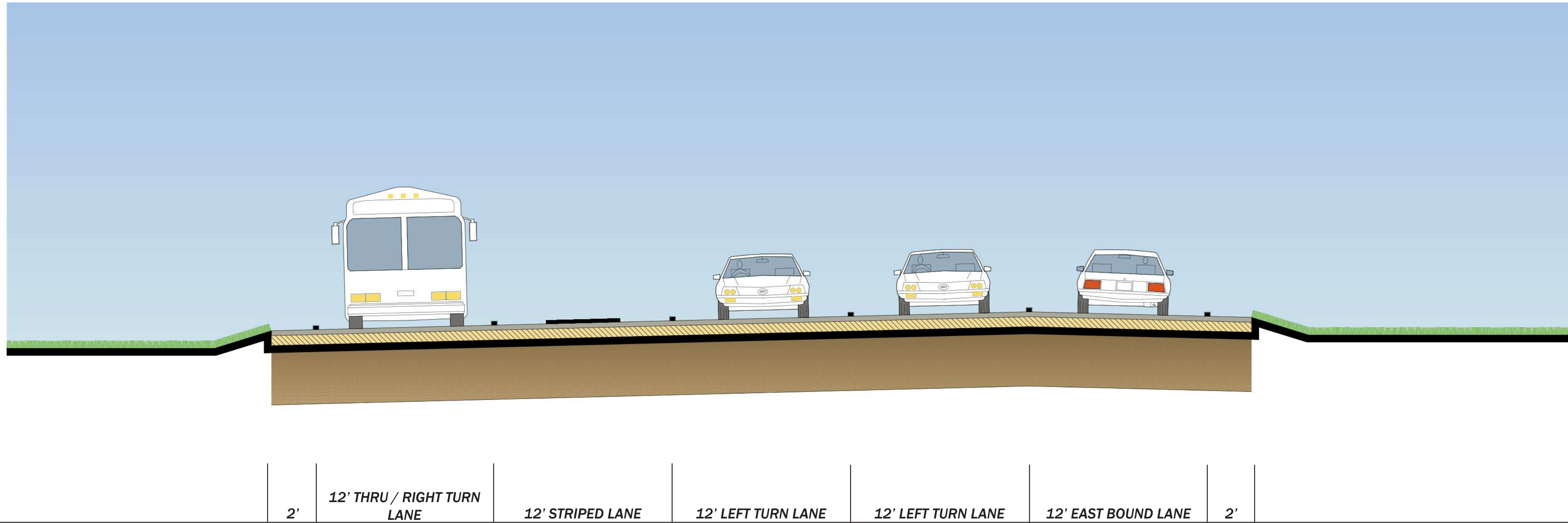
Elevation A-A - Not to Scale, for Illustration Purposes Only
