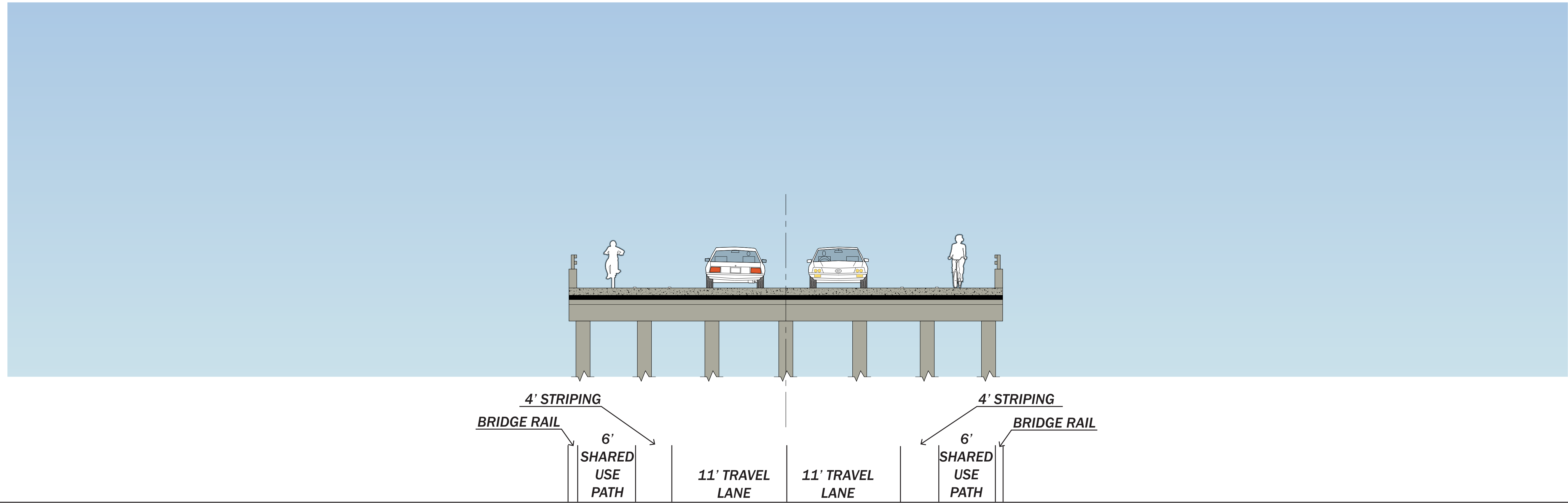
Elevation 1-1 - N Sherwood Forest Dr. Bridge - Not to Scale, for Illustration Purposes Only
