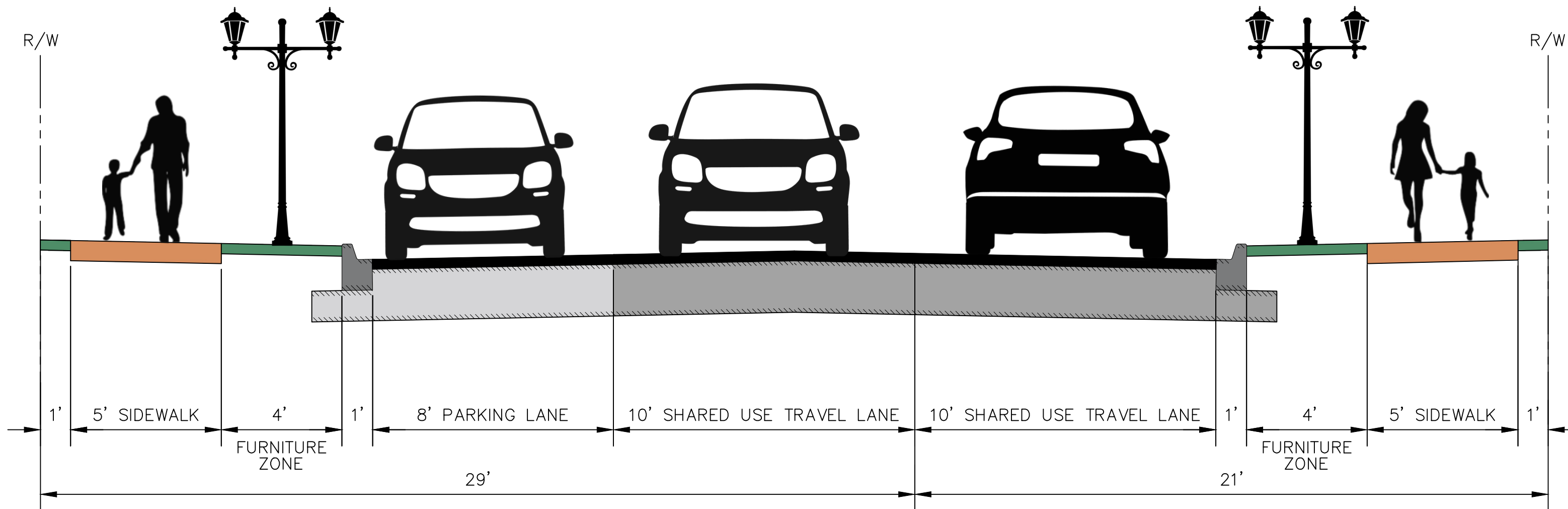
PROPOSED ROADWAY NO BIKE LANES\ON STREET PARKING
