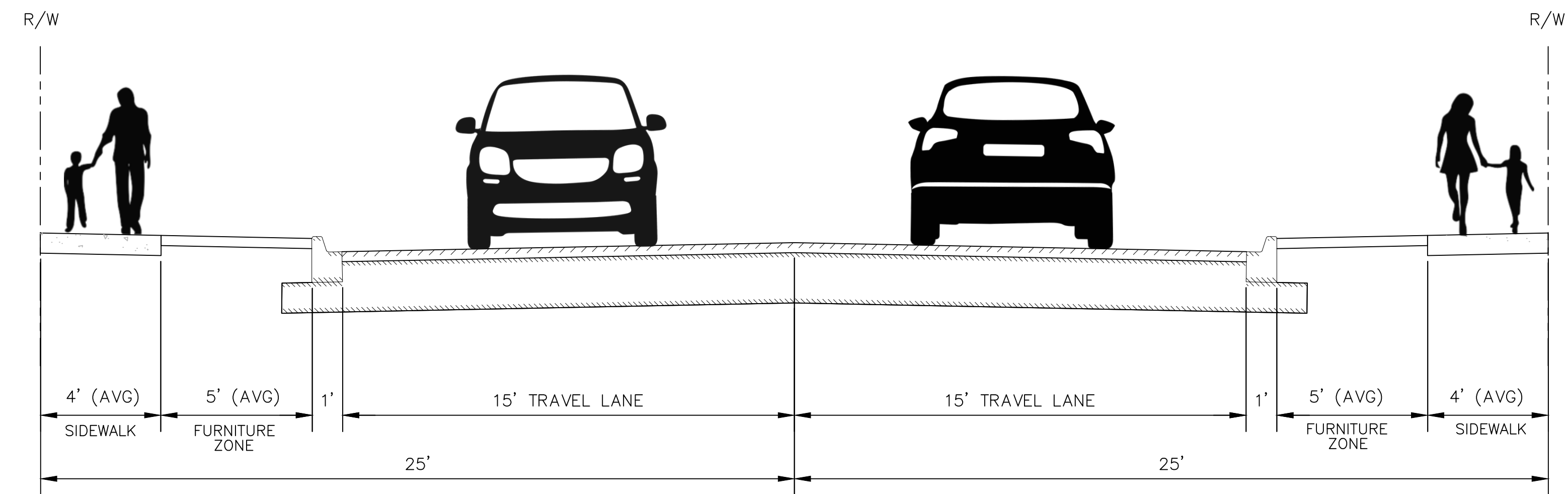
EXISTING ROADWAY
